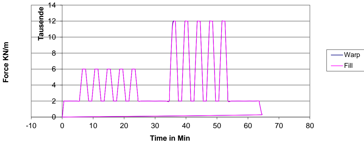
Strain - Time
