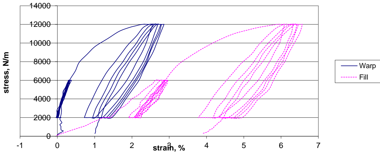
Stress-strain
